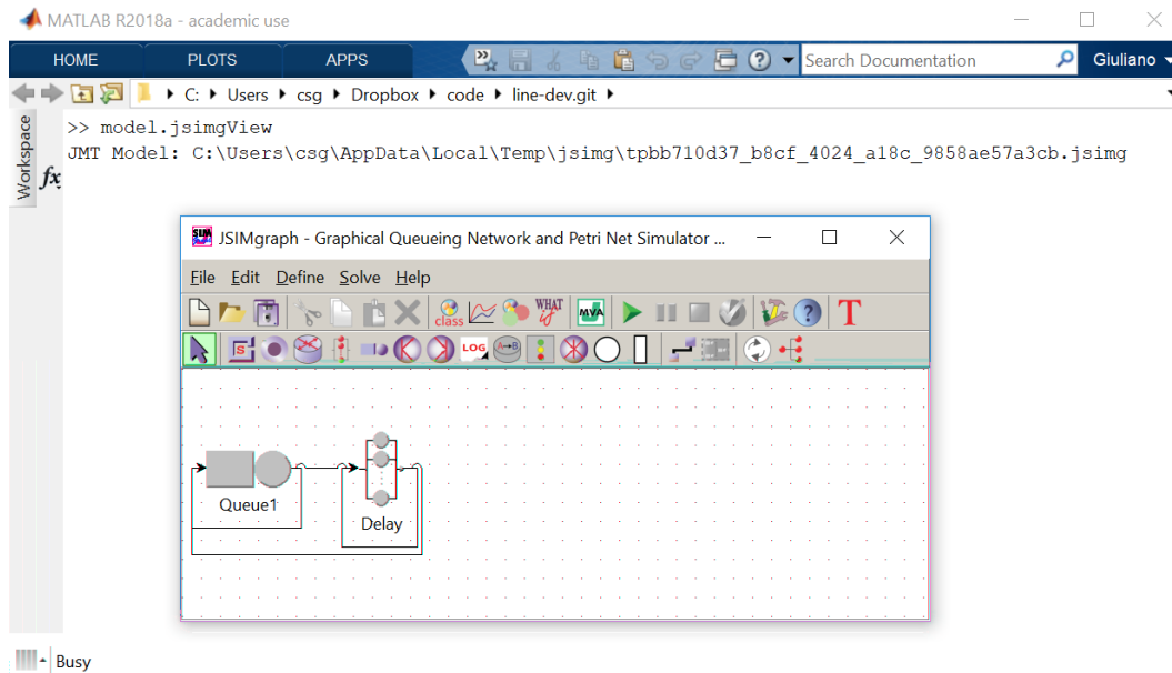
Figure 3.4: jsimView function
