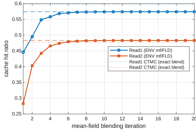
Figure 6.11: Mean-field ENV blending for the MMAP-modulated cache of Example 6.6.3. Starting from an empty cache, the per-read-class hit ratios produced by the default (mean-field) ENV analyzer with an FLD inner solver converge over the blending iteration to the environment-blended equilibrium (dashed), obtained by carrying each phase’s mean cache occupancy across phase switches. The exact CTMC blend (dotted) is approached up to the mean-field error of the small ( n=4 , m=2 ) cache.
