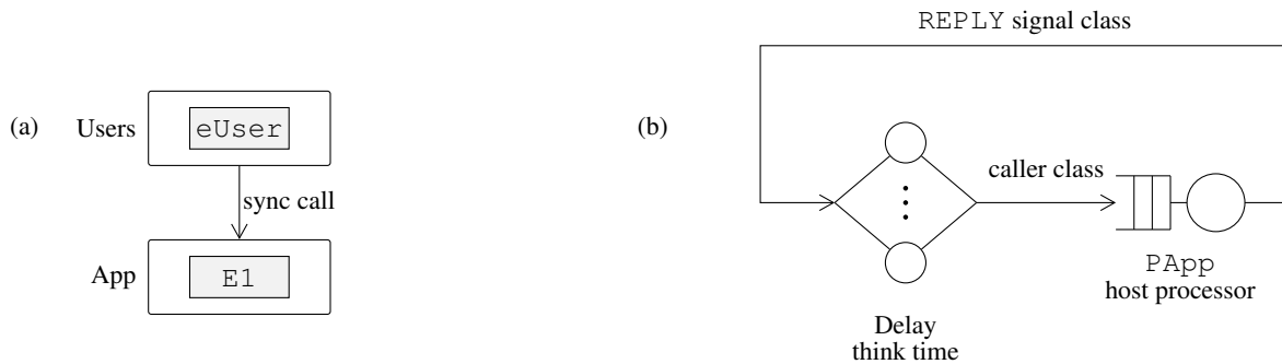
Figure 6.8: The output of LQN2QN. (a) A reference task issuing one synchronous call to an entry of a server task. (b) The flattened queueing network: the host processor of each task becomes a station, the reference task becomes a Delay holding its think time, and each step of the activity graph becomes a closed class. The caller is blocked while the callee runs, and is released by the REPLY signal class emitted by the replying activity.
