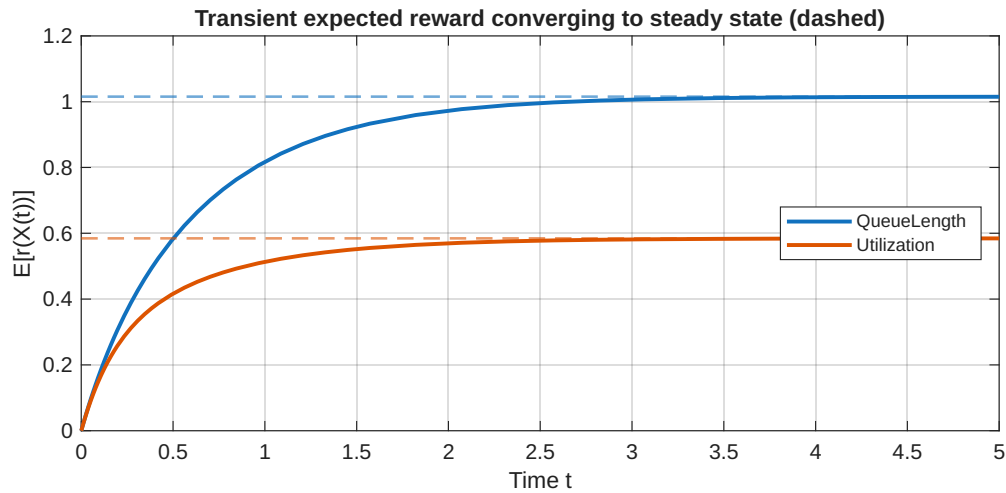
Figure 4.1: Transient expected reward E[r(X(t))] for the queue length and utilization of an M/M/1/3 queue, converging over time to the steady-state values (dashed) computed by getAvgReward .
