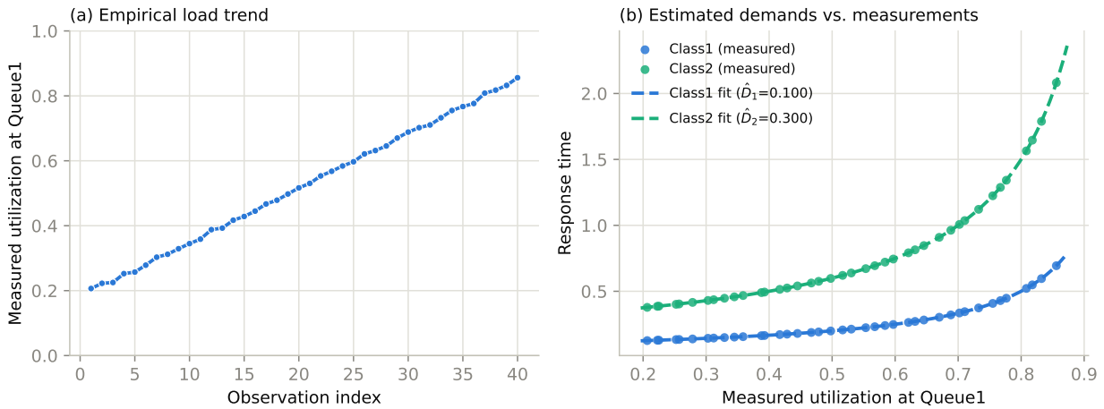
Figure 8.1: Quick-start example: (a) the empirical utilization trend as the workload ramps up over the observation window; (b) the measured response times against utilization, together with the M/G/1 curves \hat{D}_r/(1-u) reconstructed from the demands \hat{D}_1, \hat{D}_2 estimated by the UBO method.
