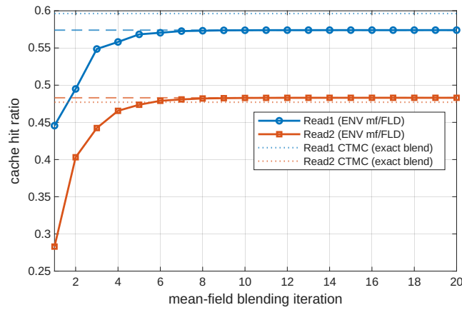
Figure 7.2: Mean-field \text{ENV} blending for the MMAP-modulated cache of Example 7.3.5. Starting from an empty cache, the per-read-class hit ratios produced by the default (mean-field) \text{ENV} analyzer with an \text{FLD} inner solver converge over the blending iteration to the environment-blended equilibrium (dashed), obtained by carrying each phase's mean cache occupancy across phase switches. The exact \text{CTMC} blend (dotted) is approached up to the mean-field error of the small ( n=4 , m=2 ) cache.
