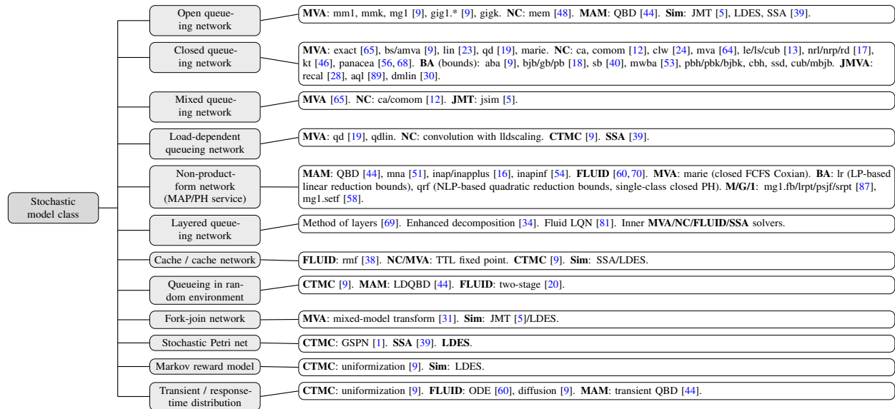
Figure 5.1: Taxonomy of solution techniques available in LINE for each class of stochastic model. Each leaf lists the short method name (as accepted by options.method ) with its bibliographic reference; entries without a reference denote simulation backends or aliases. See Table 5.1 for the solver exposing each method.
