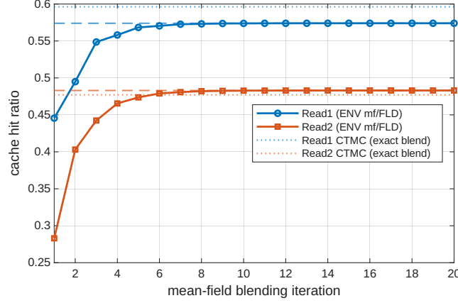
Figure 7.2: Mean-field ENV blending for the MMAP-modulated cache of Example 7.3.5. Starting from an empty cache, the per-read-class hit ratios produced by the default (mean-field) ENV analyzer with an FLD inner solver converge over the blending iteration to the environment-blended equilibrium (dashed), obtained by carrying each phase’s mean cache occupancy across phase switches. The exact CTMC blend (dotted) is approached up to the mean-field error of the small ( n=4 , m=2 ) cache.
