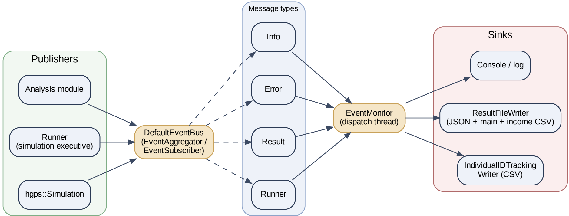
Figure 11. Event-driven messaging and output architecture
