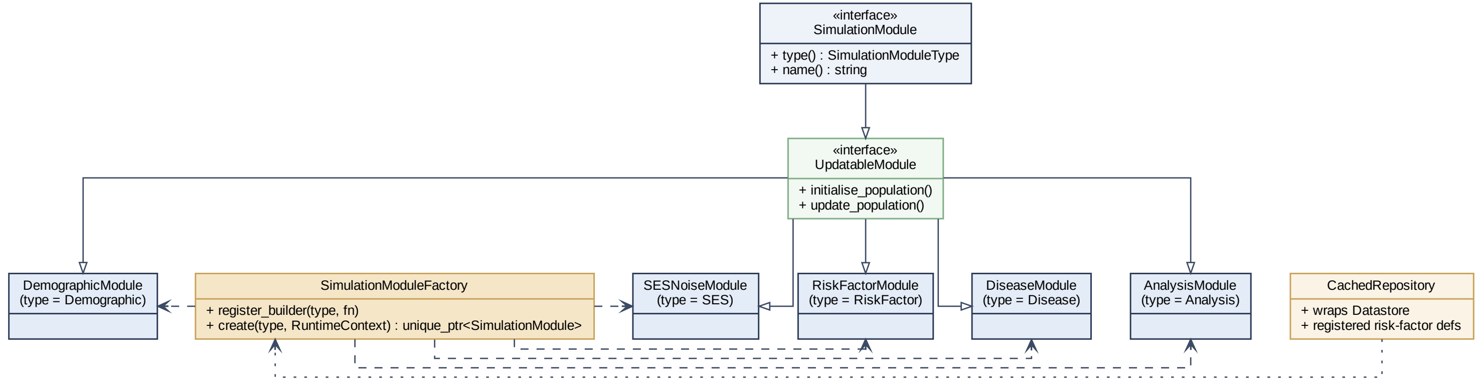
Figure 4. Common module interface and factory (src/HealthGPS/interfaces.h)
