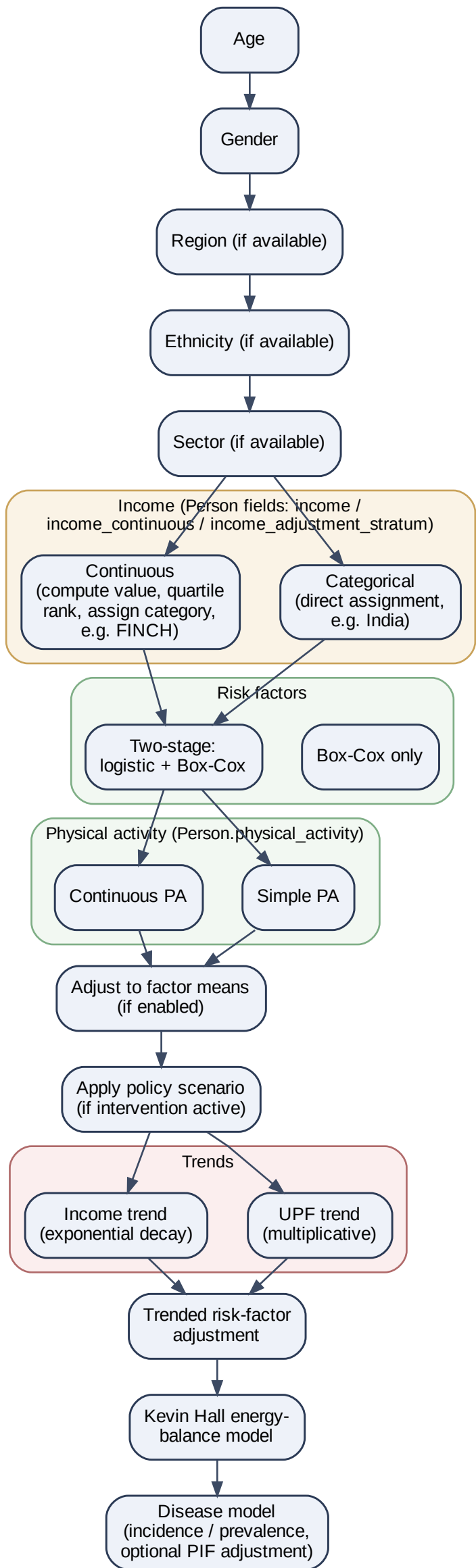
Figure 6. Per-individual initialisation sequence (initialise_population)
