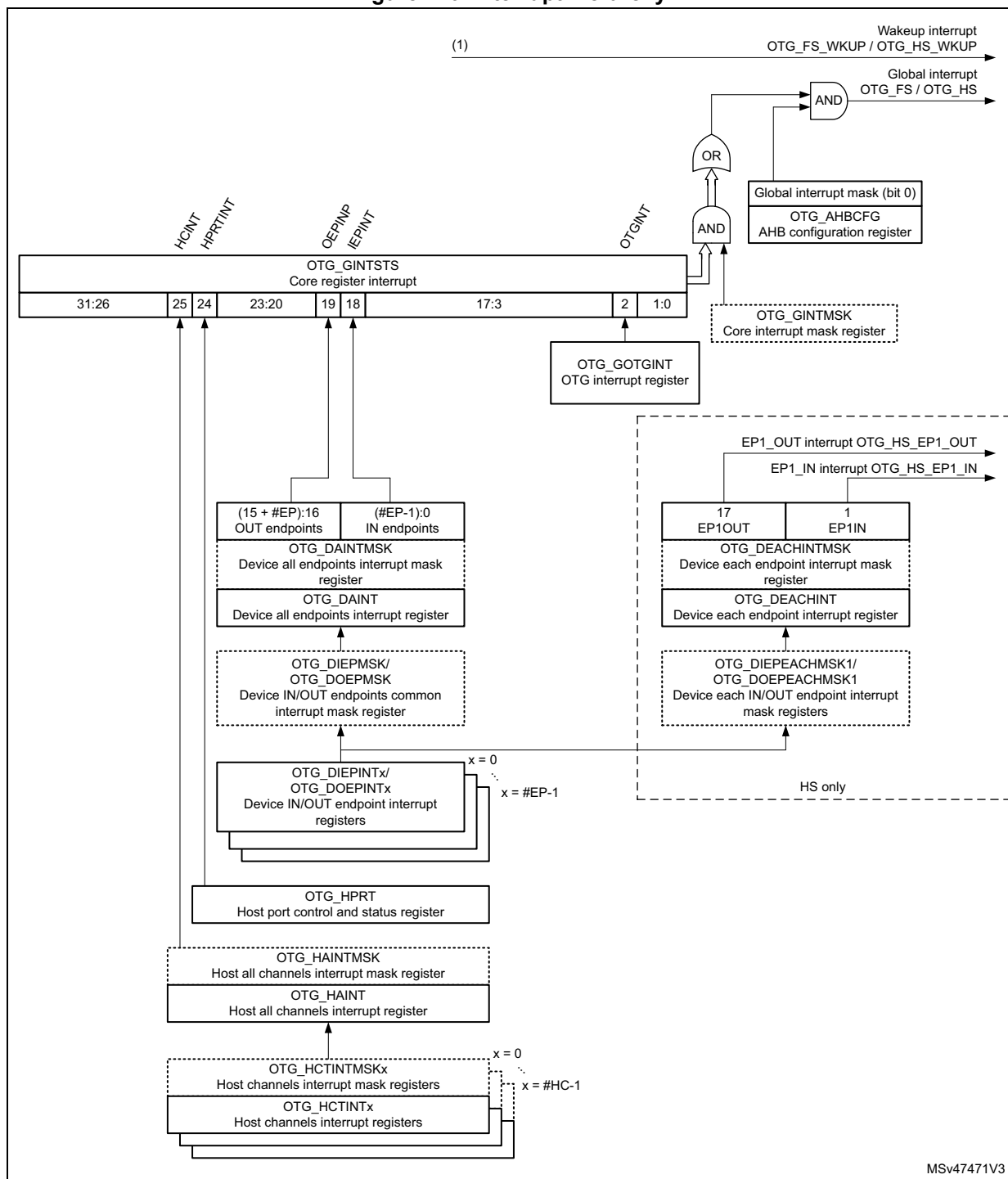
Figure 410. Interrupt hierarchy
