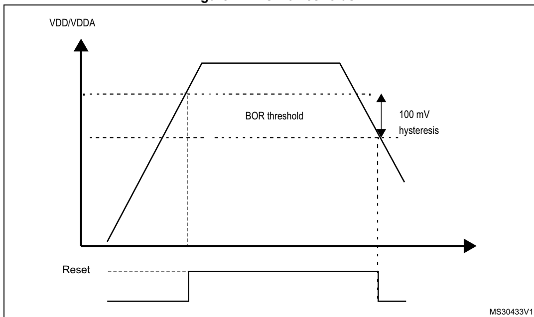
Figure 11. BOR thresholds
