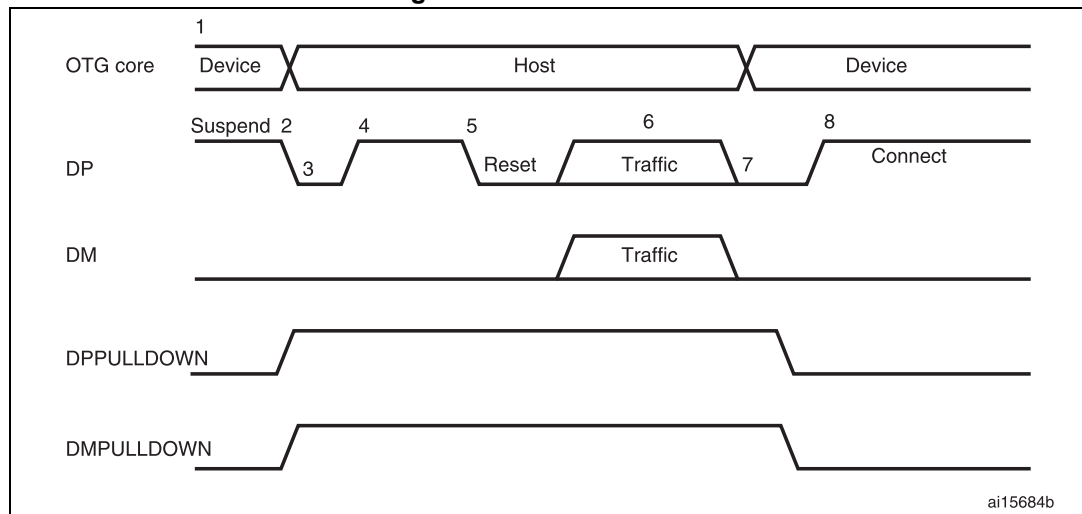
Figure 432. B-device HNP
