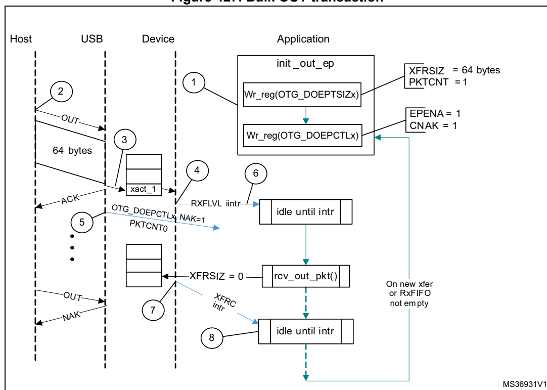
Figure 427. Bulk OUT transaction
