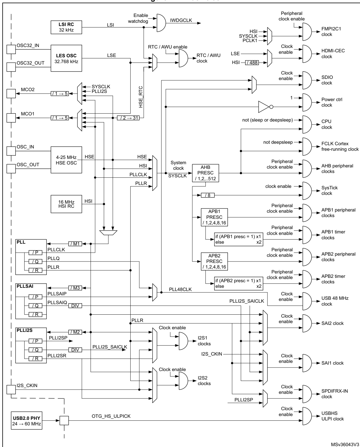
Figure 14. Clock tree
