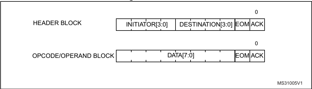
Figure 435. Blocks
