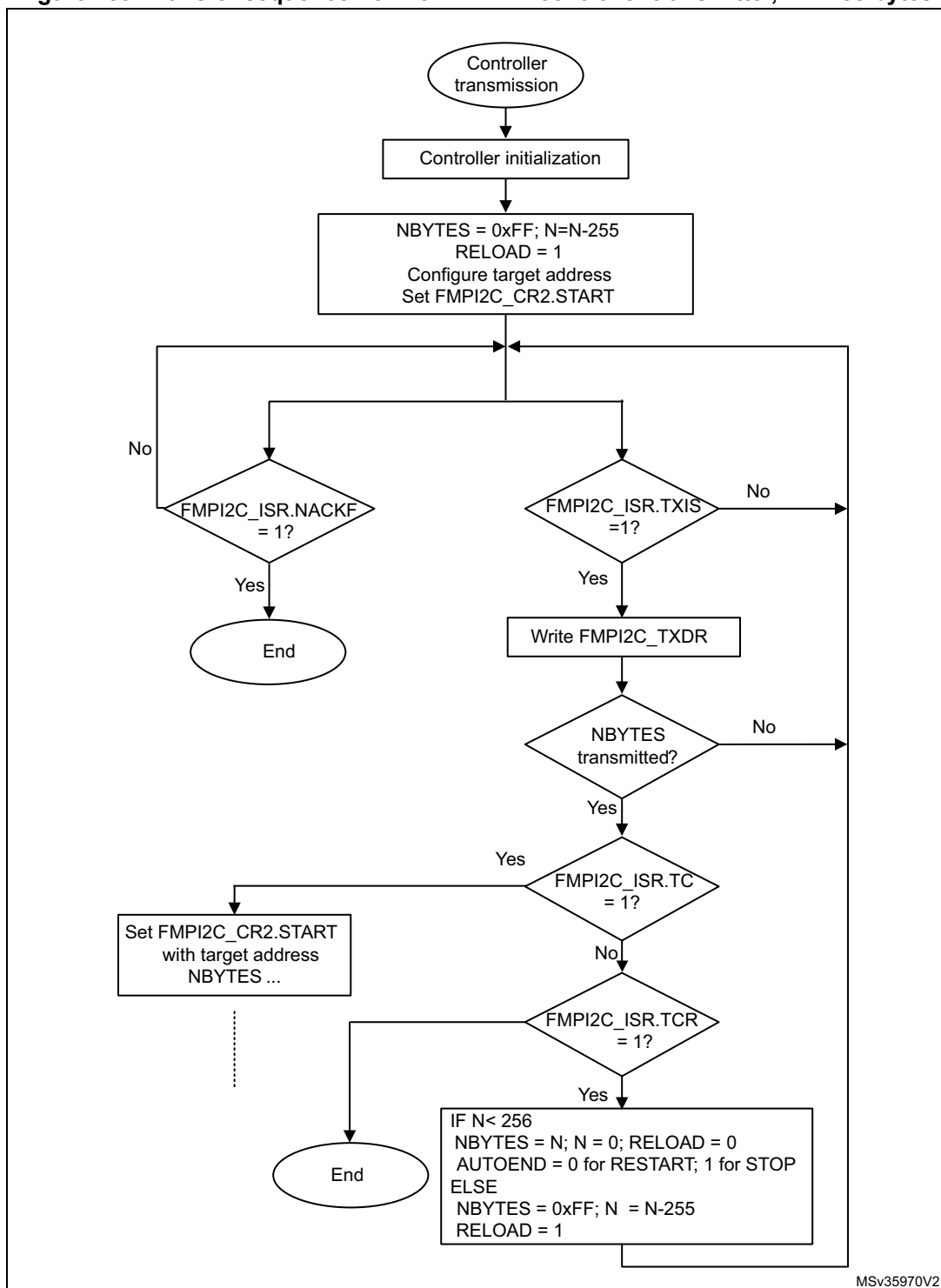
Figure 259. Transfer sequence flow for FMPI2C controller transmitter, N > 255 bytes
