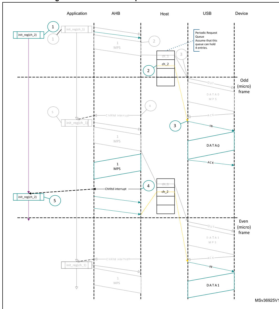
Figure 422. Normal interrupt IN transactions - DMA mode
