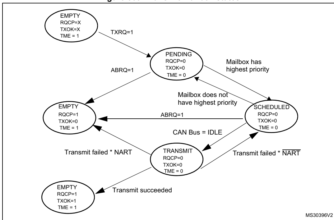
Figure 389. Transmit mailbox states
