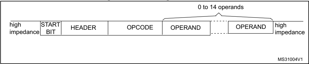
Figure 434. Message structure
