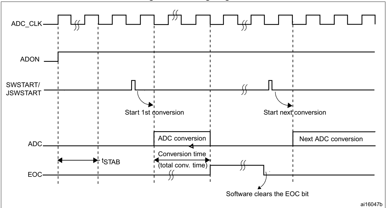
Figure 73. Timing diagram
