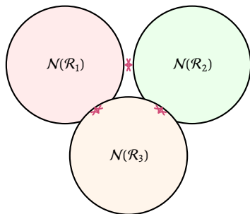
Figure 42 – Conceptual distinction between the two planes. On the left: a single nomy \mathcal{N}(\mathcal{R}) decomposed internally into an n-tuple of subnomies (\mathcal{N}_1, \dots, \mathcal{N}_n) coupled by the operator \otimes . On the right: a system of coupled realities, in which multiple parallel realities (\mathcal{R}_1, \mathcal{R}_2, \mathcal{R}_3) , each with its own nomy, interact through external channels (dashed lines). Each of these nomies may, in turn, admit its own decomposition into an internal n-tuple of subnomies.
