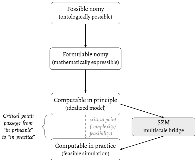
Figure 45 – Conceptual flow among the levels of accessibility of a nomy. The transition between “computable in principle” and “computable in practice” represents the critical point where the main analytical and computational barriers arise. The SZM is indicated as a potential methodological bridge to act in this region.
