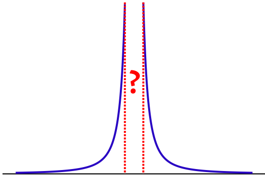
Figure 49 – Representation of the magnitude of the electric field in the vicinity of an electron. The region in blue is known: it is described by Coulomb's Law. What lies at the center, between the dotted red lines in red and marked with “?”, remains unknown.
