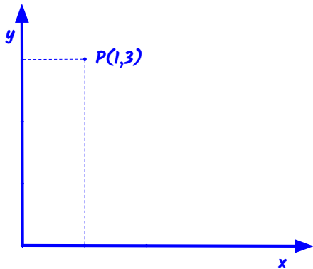
Figure 8 – Representation of the point P(1, 3) in a two-dimensional Cartesian system.
