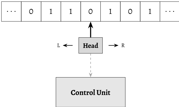
Figure 16 – Schematic representation of a Turing machine. The model consists of a potentially unbounded tape divided into cells, each containing a symbol. The head reads and writes symbols on the tape, and can move to the left (L) or right (R). The control unit determines the action to be performed based on the current state and the symbol read, defining the next state, the symbol to be written, and the direction of the move.
