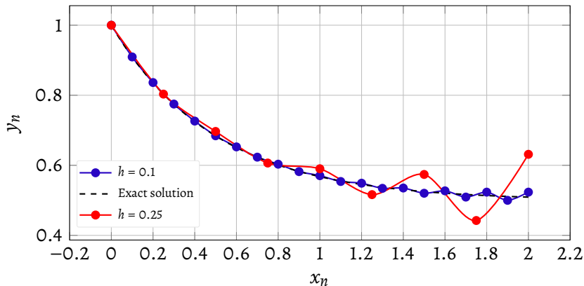
Figure 18 – Behavior of the sequence \{y_n\} for different steps h . At h = 0.1 the contamination from the spurious root does not yet dominate over the interval shown; at h = 0.25 it is already visible. The analytical solution y(x) = \frac{1}{2}(1 + e^{-2x}) is represented by the dashed curve.
