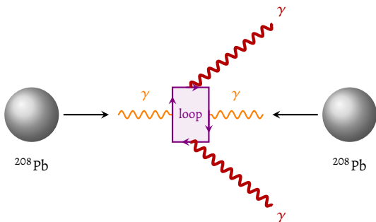
Figure 5 – Light-by-light scattering ( \gamma\gamma \rightarrow \gamma\gamma ) in ultra-peripheral Pb–Pb collisions at the LHC. Each relativistic nucleus emits a quasi-real photon; these interact via a loop of virtual fermions ( box diagram), producing two real photons in the final state ( ATLAS Collaboration, 2017 ; ATLAS Collaboration, 2019 ).
