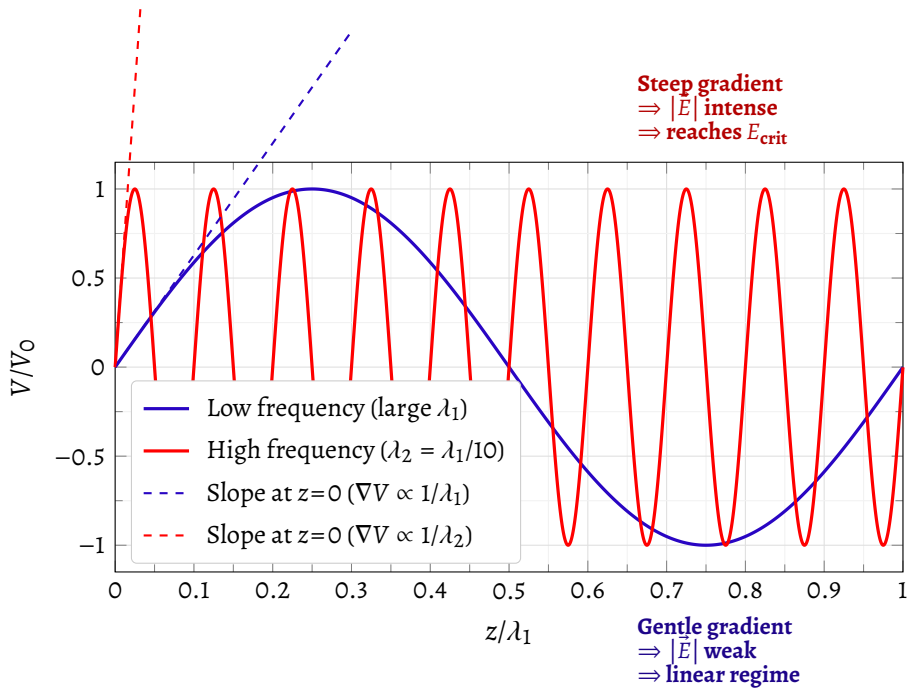
Figure 7 – Comparison of the electric potential V(z) for two waves with the same amplitude V_0 , but with different frequencies, at the instant t = 0 . The high-frequency wave (red, \lambda_2 = \lambda_1/10 ) exhibits a spatial gradient 10 times steeper than the low-frequency wave (blue). By the relation \vec{E} = -\nabla V , this results in an electric field 10 times more intense. It is precisely this effect that causes the high-frequency modes to reach E_{\text{crit}} first, activating the nonlinear suppression.
