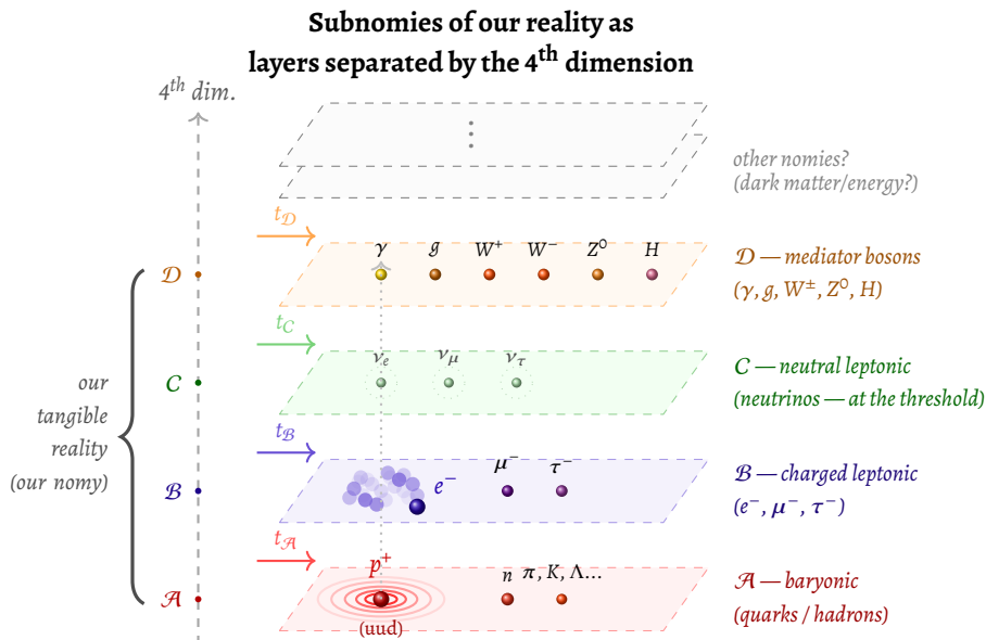
Figure 57 – Ontological layered representation of the subnomies that compose our nomy (tangible reality). Each layer corresponds to a distinct subnomy, separated from the others by the fourth dimension. In the baryonic layer \mathcal{A} , the proton p^+ (composed of uud quarks) generates an electric field with a characteristic radial profile. In the charged leptonic layer \mathcal{B} , the electron e^- occupies a specific position — unknown to an observer in layer \mathcal{A} —, represented by the cloud of ignorance (blue shadows) concentrated around the vertical projection of the proton, giving rise to the 1s orbital. Layer \mathcal{C} (neutrinos) lies at the threshold of our nomy, almost decoupled from the other subnomies. Layer \mathcal{D} houses the mediator bosons of the fundamental interactions. Each layer has its own temporal structure ( t_{\mathcal{A}}, \dots, t_{\mathcal{D}} ), disconnected from the others. Above the brace are indicated, hypothetically, other nomies possibly not detectable by our instruments — possibly associated with dark matter and dark energy.
