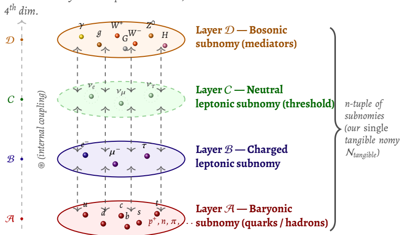
Figure 58 – Schematic representation of our tangible nomy N_{\text{tangible}} as an n-tuple of subnomies , arranged in distinct ontological layers: \mathcal{A} (baryonic), \mathcal{B} (charged leptonic), \mathcal{C} (neutral leptonic, at the threshold), and \mathcal{D} (bosonic). The vertical dashed arrows represent the coupling \otimes between subnomies, encoding the structure \mathcal{K} = (\mathcal{M}, \mathcal{R}, \mathcal{A}) of mixing, shared representation, and anomaly conditions (Chapter 14). Crucial observation: the disks do NOT represent independent parallel realities, but rather sectors (subnomies) of the same tangible nomy , internally coupled. The proton–electron interaction (Figures 54 and 55) manifests itself as the coupling \mathcal{A} \otimes \mathcal{B} .
