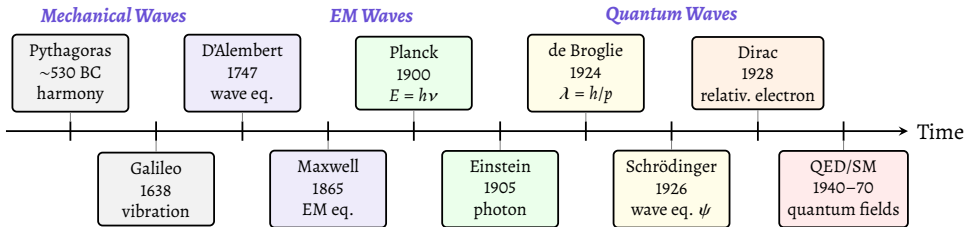
Figure 60 – Timeline of the contributions that led from mechanical waves to quantum mechanics and the Standard Model. Each color transition represents a change of wave paradigm — or, in the language of this book, a change of nomy .
