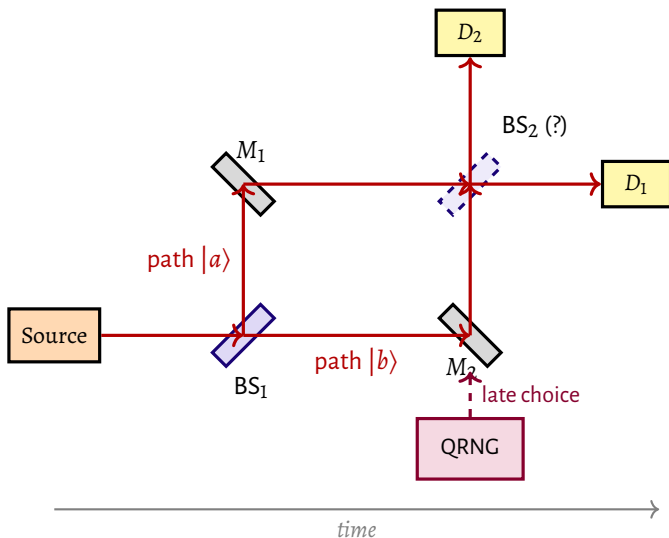
Figure 11 – Schematic of the delayed-choice experiment (Mach-Zehnder version). A photon emitted by the source strikes the beam splitter BS_1 , creating a coherent superposition of the paths |a\rangle (via mirror M_1 ) and |b\rangle (via mirror M_2 ). Crucial decision: after the photon has already passed through BS_1 and is in the arms of the interferometer, a quantum random number generator (QRNG) decides whether the second splitter BS_2 will be present or absent. If BS_2 is present , the paths recombine and the photon exhibits interference (wave behavior) — detectors D_1 and D_2 register counts with probabilities depending on the relative phase between the arms. If BS_2 is absent , each detector is connected uniquely to one of the paths, revealing a definite trajectory (particle behavior). Wheeler’s question was: how does the photon “know” which behavior to adopt if the decision was made after it had already entered the interferometer?
