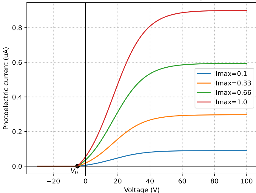
Figure 13 – Photoelectric current as a function of voltage for different light intensities at the same frequency.
