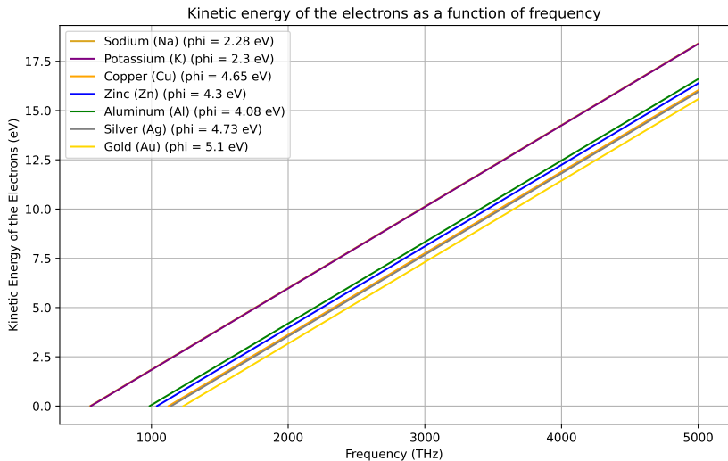
Figure 14 – Kinetic energy of the emitted photoelectrons as a function of the light frequency for different metals.
