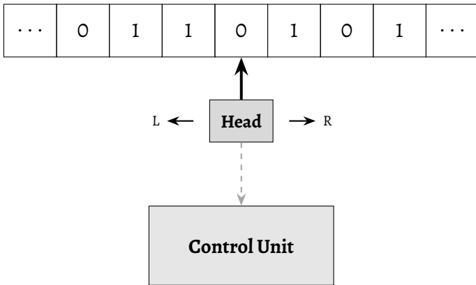
Figure 15 – Schematic representation of a Turing machine. The model consists of a potentially unbounded tape divided into cells, each containing a symbol. The head reads and writes symbols on the tape, and can move to the left (L) or right (R). The control unit determines the action to be performed based on the current state and the symbol read, defining the next state, the symbol to be written, and the direction of the move.
