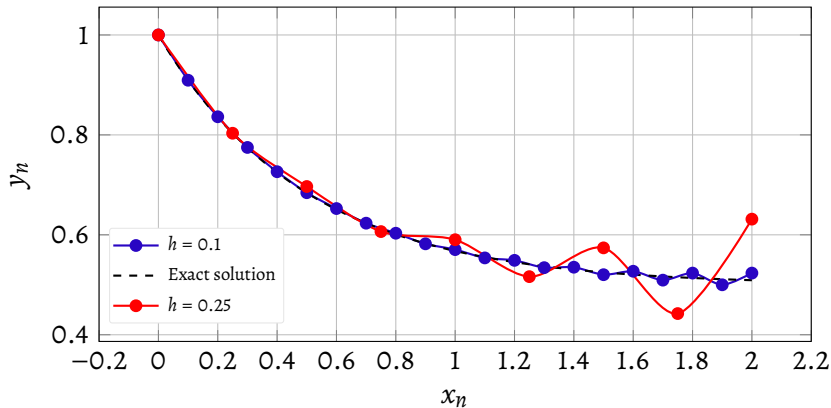
Figure 17 – Behavior of the sequence \{y_n\} for different steps h . At h = 0.1 the contamination from the spurious root does not yet dominate over the interval shown; at h = 0.25 it is already visible. The analytical solution y(x) = \frac{1}{2}(1+e^{-2x}) is represented by the dashed curve.
