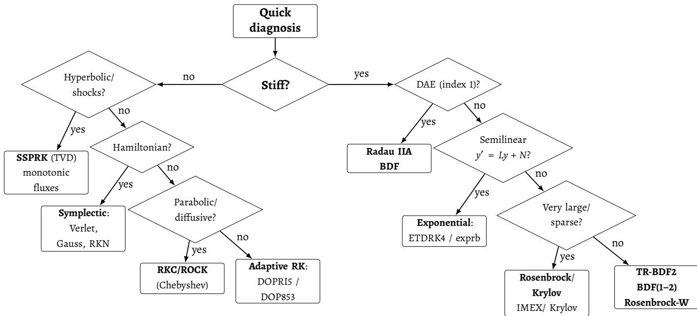
Figure 20 – Flowchart for selecting the most suitable numerical method for integrating ODEs, starting from the identification of the stiffness of the problem.
