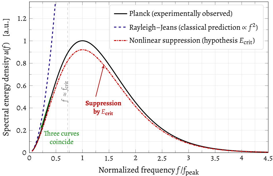
Figure 8 – Qualitative comparison between the classical Rayleigh–Jeans prediction (dashed blue, u \propto f^2 , divergent), the experimentally observed Planck distribution (solid black), and the behavior intended by the nonlinear-suppression hypothesis (red dash-dot; an illustration, not a result computed from the hypothesis). When the electric field of the high-frequency modes reaches E_{\text{crit}} , the restitutive nonlinearity prevents the indefinite accumulation of energy, producing a natural cutoff at high frequencies qualitatively compatible with the Planck curve. Compare with Figure 12 of Appendix Q.
