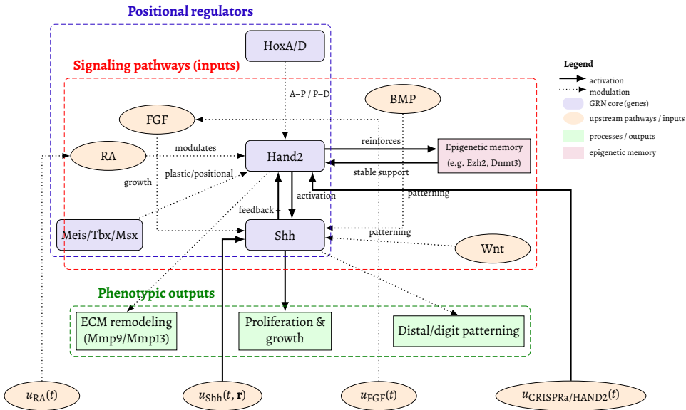
Figure 15 – Expanded GRN of axolotl regeneration: Hand2–Shh core (positive feedback) coupled to RA/FGF/BMP/Wnt pathways, positional regulators (HoxA/D, Meis/Tbx/Msx), epigenetic memory (Ezh2/Dnmt3), and morphofunctional outputs. Experimental inputs u(\cdot) enable control synthesis for positional reprogramming.
