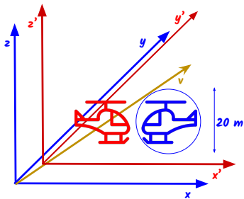
Figure 22 – Two three-dimensional helicopters 1 flying over their respective 3D spaces, but each space (or universe) is set apart from the other by a few nanometers along the fourth dimension v . The helicopters are sized such that they would fit inside a sphere 20 meters in diameter.
