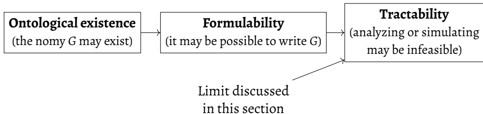
Figure 47 – Synthetic version of the hierarchy of accessibility of a nomy. The limit discussed in this section lies at the level of tractability : a nomy G may exist and be formulable, yet remain analytically or numerically intractable. For the expanded version, which details the passage between computable in principle and computable in practice , cf. Figure 45.
