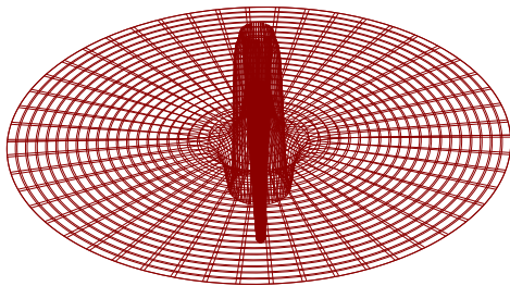
(a) Simplistic model of a hydrogen atom.
