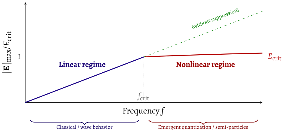
Figure 11 – Schematic diagram of the maximum amplitude of the electric field as a function of frequency, for a given potential amplitude V_0 . In the linear regime ( f < f_{\text{crit}} ), |\vec{E}| grows proportionally to f (blue line). Upon reaching E_{\text{crit}} , the restitutive nonlinearity comes into play and limits the growth of the field (red curve), forming localized excitations. The dashed gray line indicates what would occur without suppression.
