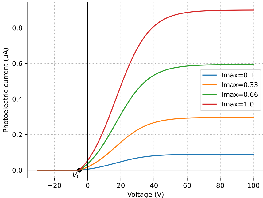
Figure 14 – Photoelectric current as a function of voltage for different light intensities at the same frequency.
