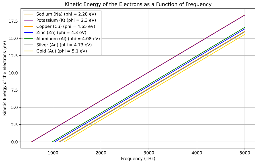
Figure 15 – Kinetic energy of the emitted photoelectrons as a function of the light frequency for different metals.
