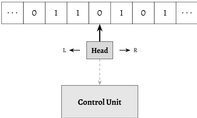
Figure 16 – Schematic representation of a Turing machine. The model consists of an infinite tape divided into cells, each containing a symbol. The head reads and writes symbols on the tape, and can move to the left (L) or right (R). The control unit determines the action to be performed based on the current state and the symbol read, defining the next state, the symbol to be written, and the direction of the move.
