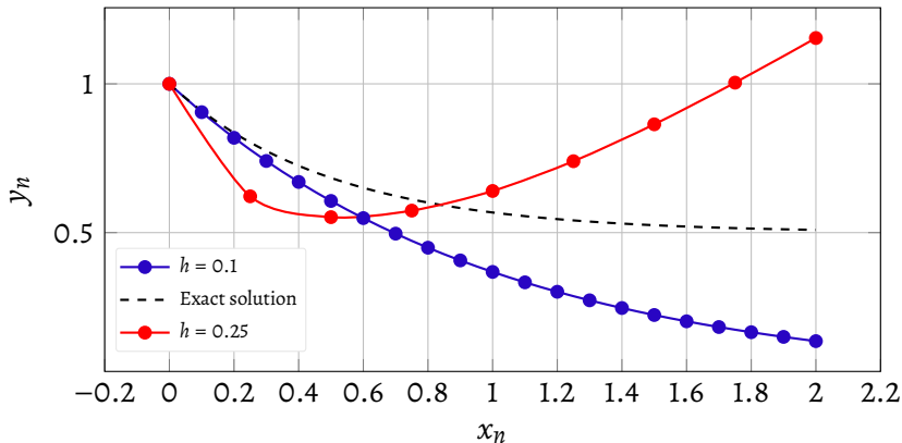
Figure 18 – Behavior of the sequence \{y_n\} for different steps h . The method is stable for h = 0.1 and becomes unstable for h = 0.25 . The analytical solution y(x) = \frac{1}{2}(1 + e^{-2x}) is represented by the dashed curve.
