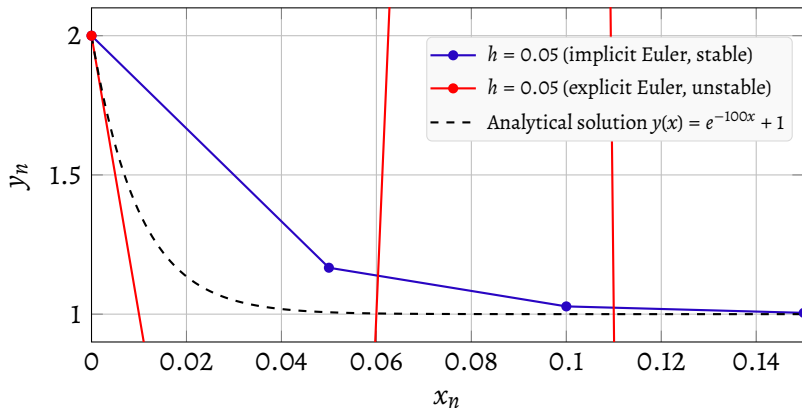
Figure 20 – Numerical stiffness in the equation y' = -100y + 100 , y(0) = 2 , with the same step h = 0.05 in two distinct methods. The explicit Euler method (red curve) is numerically unstable and generates values that blow up in magnitude and switch sign at each iteration. The implicit Euler method (blue curve), on the other hand, remains stable and approaches y = 1 rapidly, in agreement with the analytical solution (dashed curve). This contrast shows why stiff problems require implicitly stable methods.
