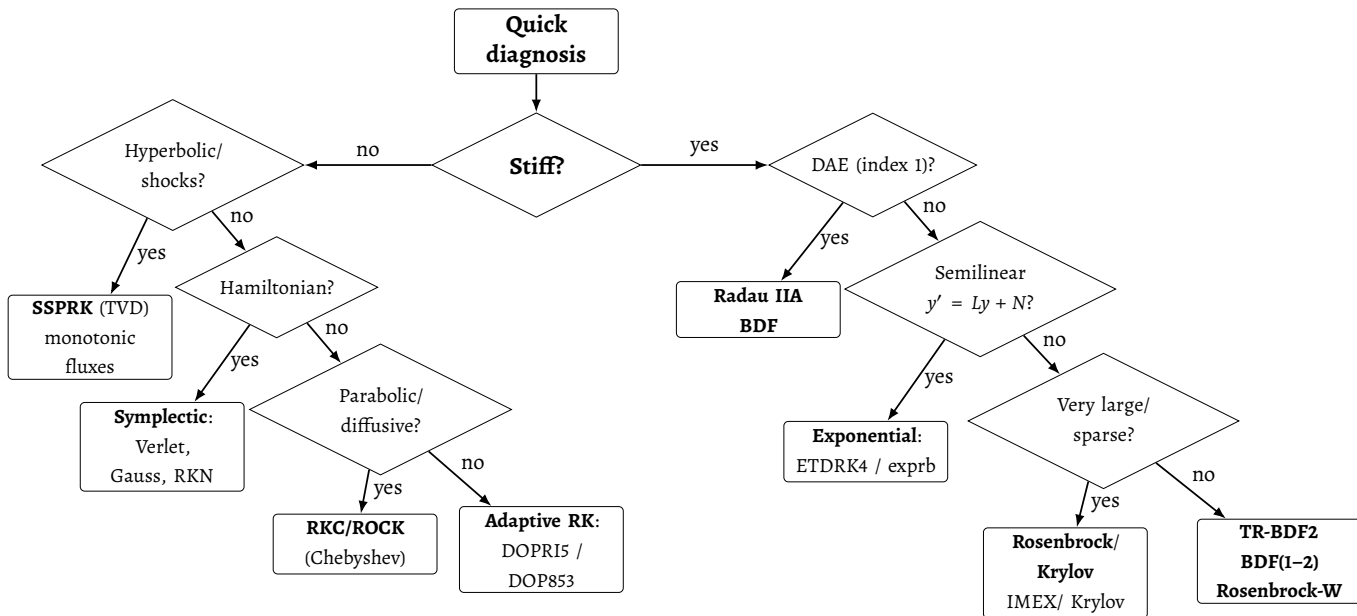
Figure 21 – Selection map (flowchart) of the most suitable numerical algorithm to solve the ODE-solving problem, starting from the identification of the stiffness of the problem.
