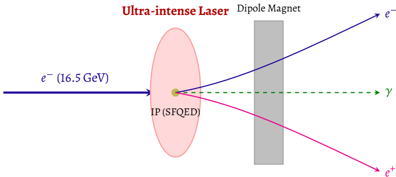
Figure 4 – Scheme of the LUXE experiment: collision between 16.5 GeV electrons and an ultra-intense laser at the interaction point (IP). After the interaction, a dipole magnet separates the products — scattered electrons ( e^- ), photons ( \gamma ), and positrons ( e^+ ) — allowing their independent detection.
