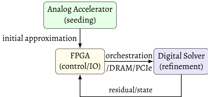
Figure 10 – Role of the FPGA in the hybrid flow: orchestration between analog seeding and digital refinement.
