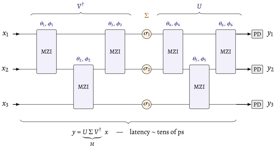
Figure 11 – Conceptual scheme of a 3 \times 3 one-shot photonic solver based on the SVD decomposition. The three horizontal lines represent waveguides. Each “MZI” rectangle is a Mach–Zehnder interferometer that couples two adjacent waveguides by means of phase shifters ( \theta, \phi ); the circles \sigma_i are optical attenuators that implement the singular values; and “PD” denotes the output photodetectors.
