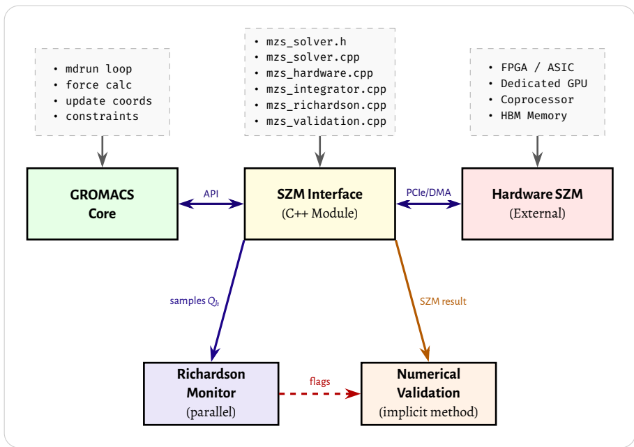
Figure 16 – SZM-GROMACS integration architecture, including modules for Richardson monitoring and numerical validation.
