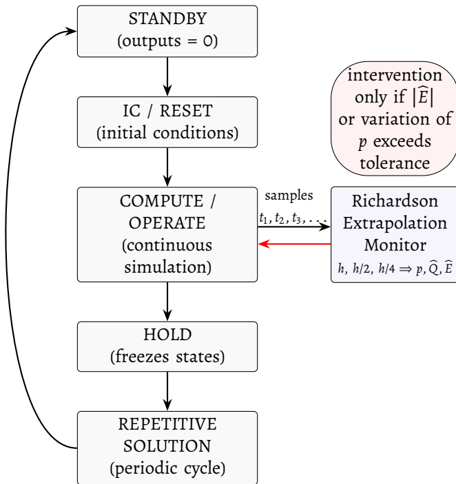
Figure 7 – Operation flow of the “analog run,” considering a classical analog computation model, adapted for parallel monitoring.
