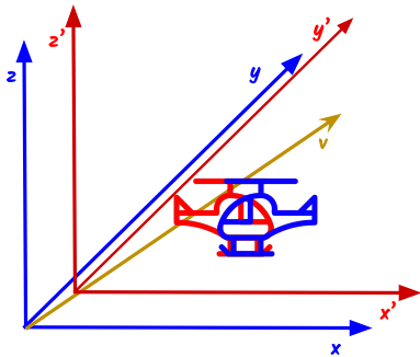
Figure 23 – Two three-dimensional helicopters almost entirely superimposed in their respective 3D spaces, but each space (or universe) is set apart from the other by fractions of a nanometer along the fourth dimension v .
