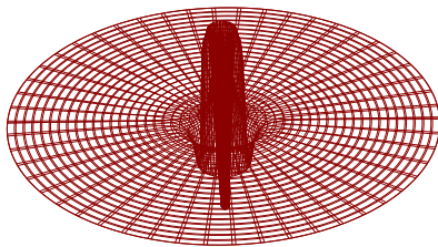
(a) Simplistic model of a hydrogen atom.
