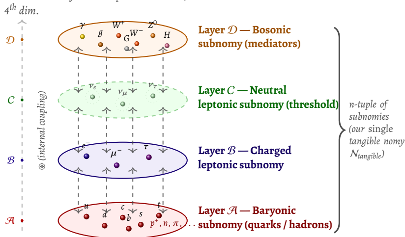
Figure 59 – Schematic representation of our tangible nomy N_{\text{tangible}} as an n-tuple of subnomies , arranged in distinct ontological layers: \mathcal{A} (baryonic), \mathcal{B} (charged leptonic), \mathcal{C} (neutral leptonic, at the threshold), and \mathcal{D} (bosonic). The vertical dashed arrows represent the coupling \otimes between subnomies, encoding the structure \mathcal{K} = (\mathcal{M}, \mathcal{R}, \mathcal{A}) of mixing, shared representation, and anomaly conditions (Chapter 14). Crucial observation: the disks do NOT represent independent parallel realities, but rather sectors (subnomies) of the same tangible nomy , internally coupled. The proton–electron interaction (Figures 54 and 56) manifests itself as the coupling \mathcal{A} \otimes \mathcal{B} .
