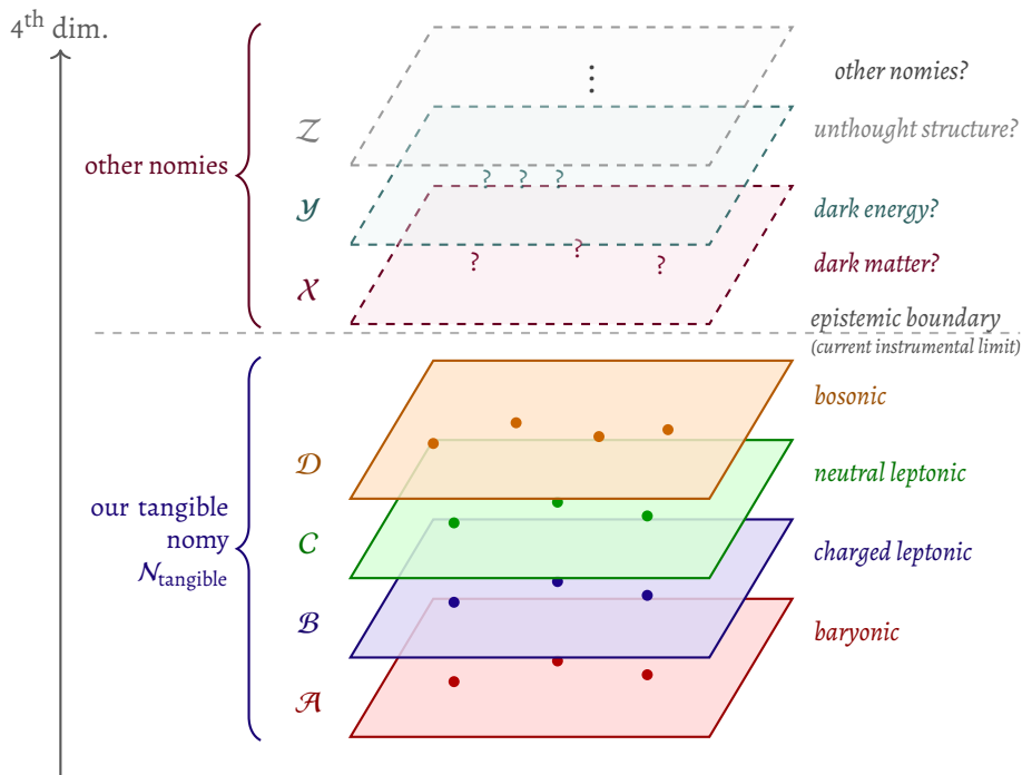
Figure 60 – Speculative extension of the layered representation along the fourth dimension (cf. Figure 58). Below the epistemic boundary, the four subnomies of our tangible nomy N_{\text{tangible}} are stacked: \mathcal{A} (baryonic), \mathcal{B} (charged leptonic), \mathcal{C} (neutral leptonic), and \mathcal{D} (bosonic) — solid layers, detectable by current instruments. Above the epistemic boundary (horizontal dashed line), dashed and progressively faded layers represent hypothetical nomies: \mathcal{X} could correspond, speculatively, to dark matter; \mathcal{Y} , to dark energy; \mathcal{Z} and the layers above represent structures still unthought or inaccessible. The epistemic boundary is historical and instrumental : should fundamental particles unknown today come to be discovered, we adopt, by convention, that they will inhabit layers distinct from \mathcal{A}, \mathcal{B}, \mathcal{C}, \mathcal{D} — that is, outside the tangible nomy as defined in this book. This figure does not represent parallel realities in Everett’s sense: the layers illustrated here coexist in the same 4th dimension, but are mutually inaccessible to the instruments typical of each nomy.
