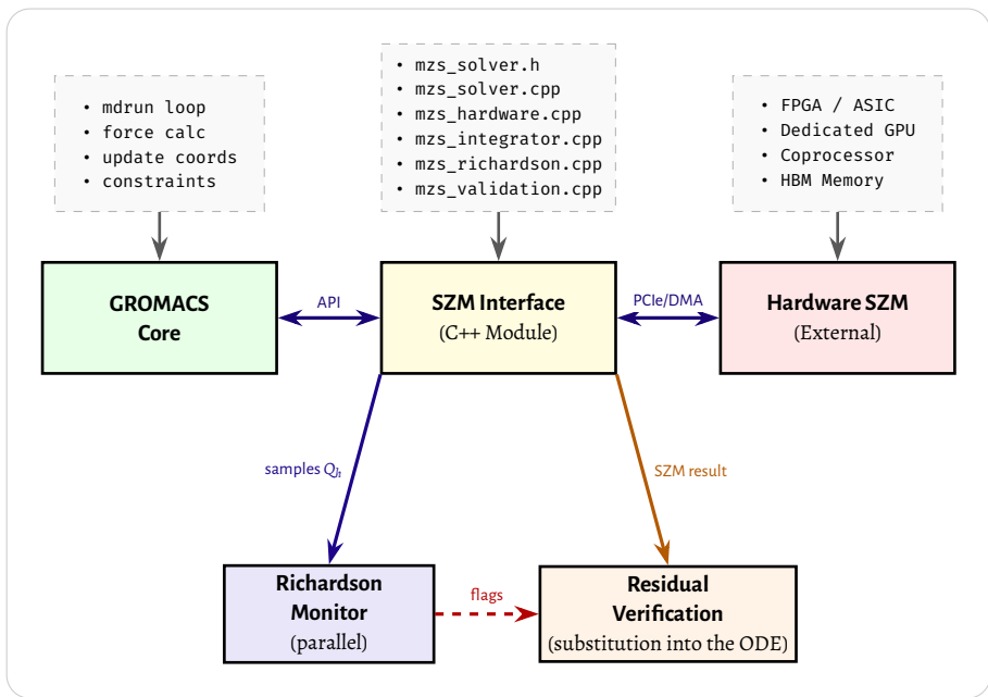
Figure 17 – SZM-GROMACS integration architecture, including modules for Richardson monitoring and numerical validation.
