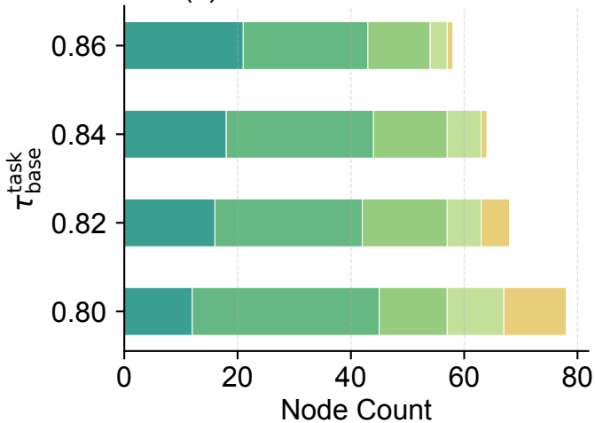
(c) SciWorld — Task Tree
