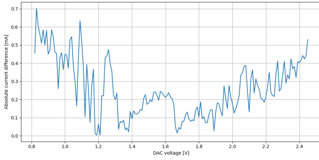
Fig. 8. Absolute current spread between loads as a function of DAC voltage in the selected valid operating region.
