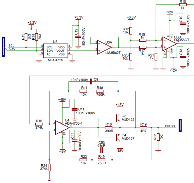
Fig. 1. Evaluated DAC and Howland-current-source output stage extracted from the STIMGRASP dissertation documentation. The schematic is used to identify the characterized circuit block and does not imply a hardware redesign.
