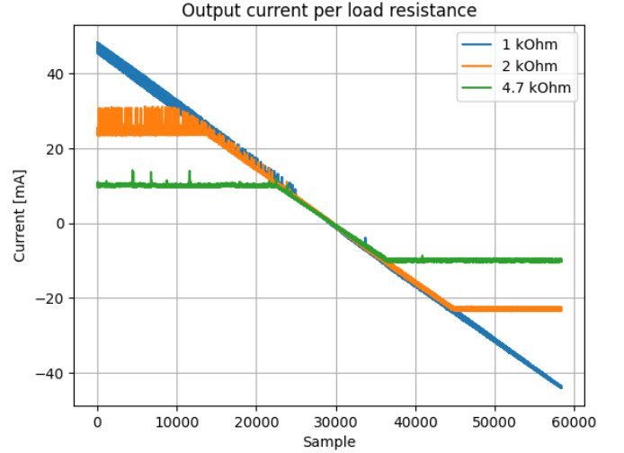
Fig. 3. Calculated output current signals for the 1\ \text{k}\Omega , 2\ \text{k}\Omega , and 4.7\ \text{k}\Omega loads obtained from the shunt voltage measurements.
