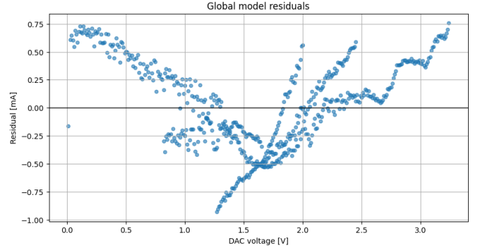
Fig. 7. Residuals of the global linear model in the selected valid operating region.
