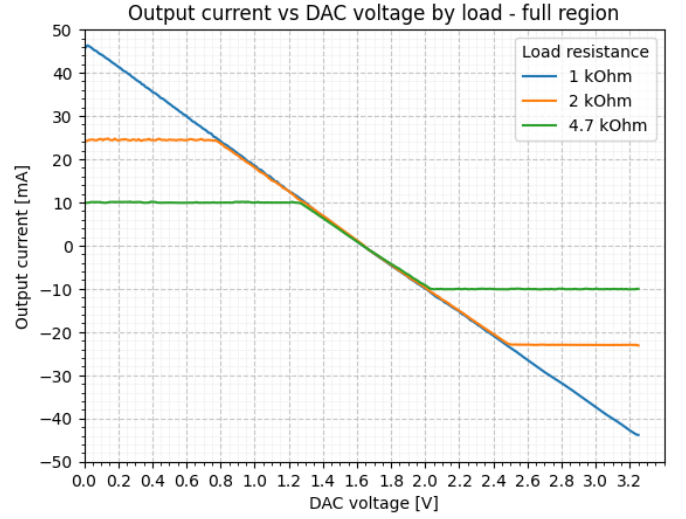
Fig. 4. Output current versus DAC voltage after reduction of signal granularity, still including the resting regime.
