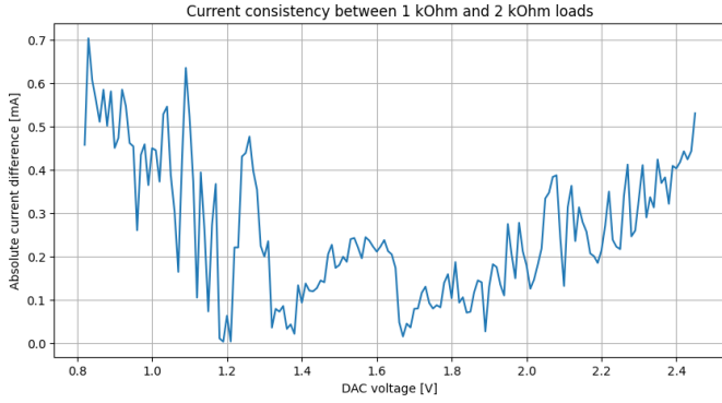
Fig. 8. Absolute current spread between loads as a function of DAC voltage in the selected valid operating region.
