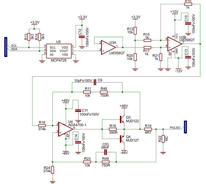
Fig. 1. Evaluated DAC and Howland-current-source output stage extracted from the STIMGRASP dissertation documentation.
