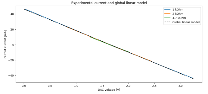
Fig. 6. Experimental current curves for 1 k \Omega , 2 k \Omega , and 4.7 k \Omega loads with the dashed global linear model identified from all loads in the valid operating region.
