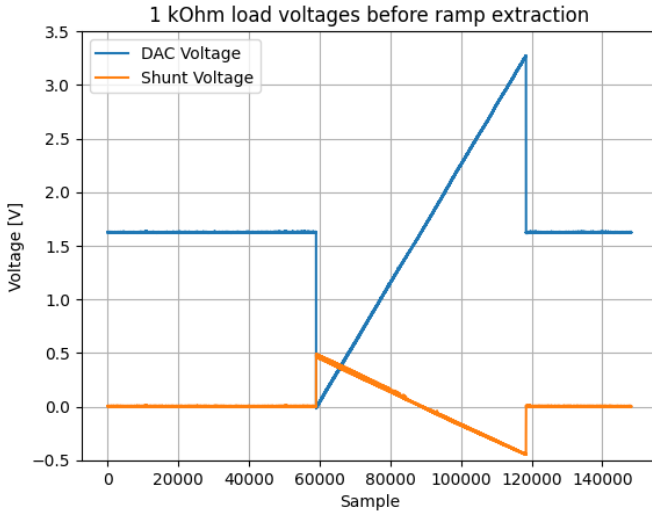
Fig. 2. Representative raw oscilloscope acquisition showing DAC voltage and shunt voltage before data treatment. The resting intervals before and after the DAC ramp are preserved in the raw CSV.
